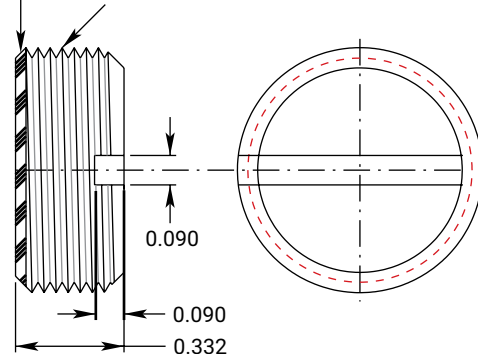
Frelon® Bearing Surface (Approx. 0.025 thick) 3/4 - 20 CLASS #2 Thread
