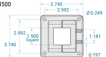
Flange Base PBH1500
